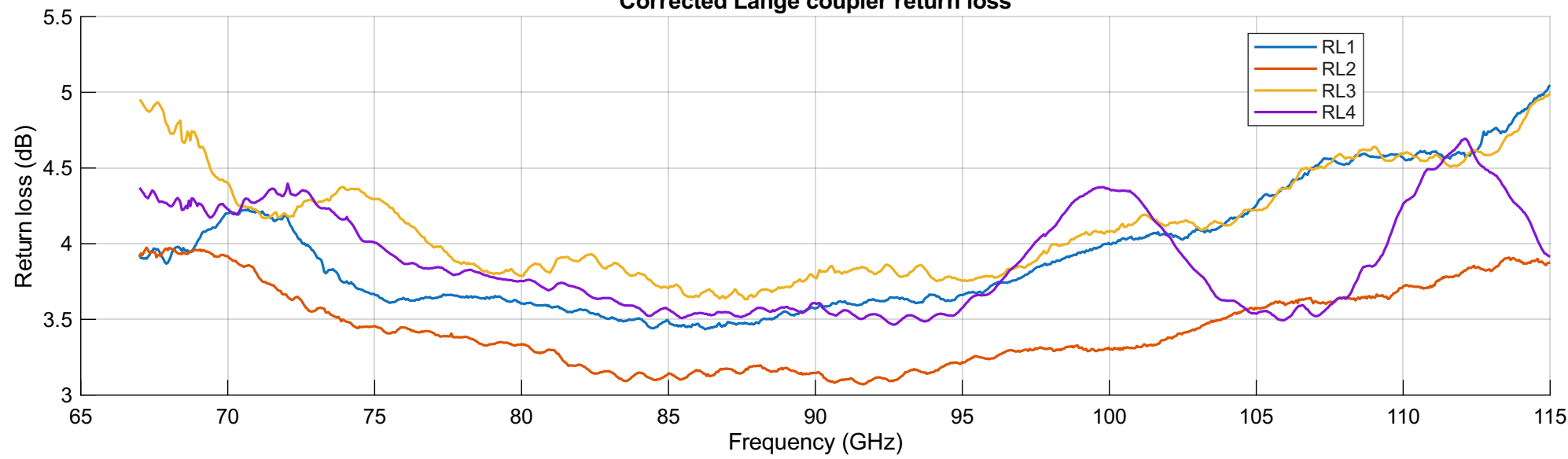
Corrected Lange coupler return loss
